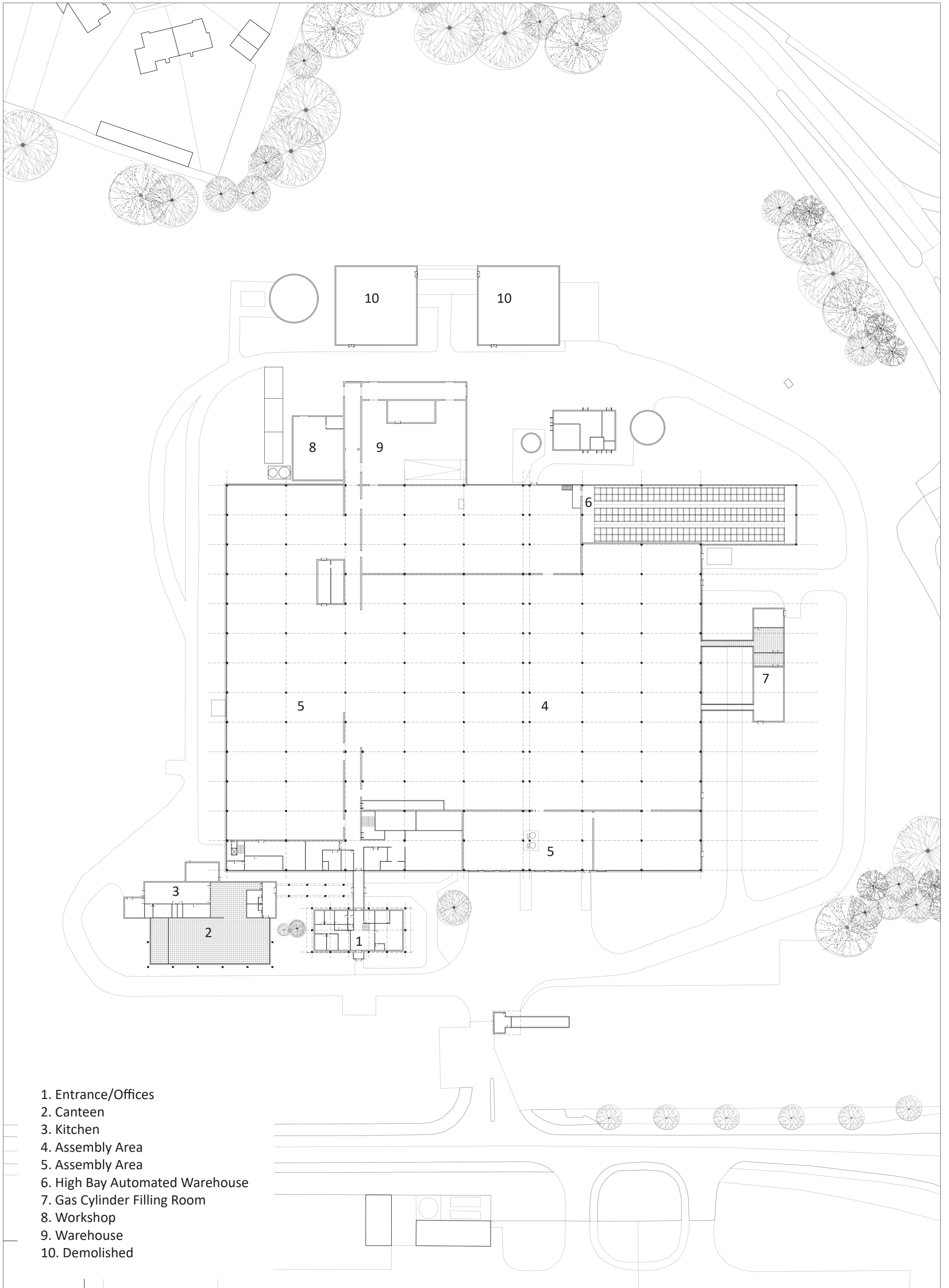
Ground Floor Plan May 2021
